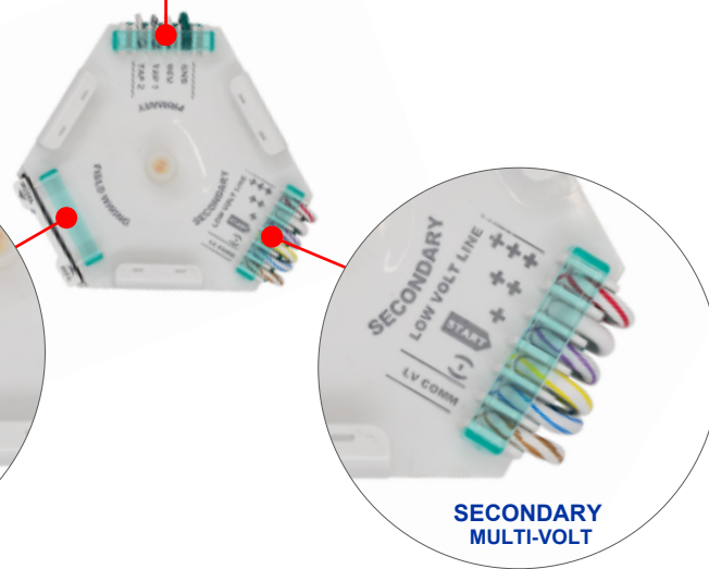
FIELD WIRING
