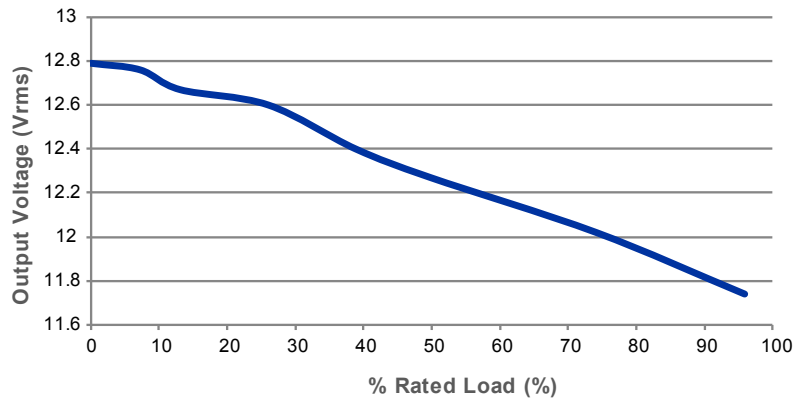
Q-HEX-300-120/12 Output Voltage vs. % Load
