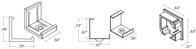
Plastic Mounting Clip
