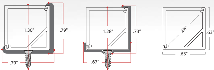
Extrusion with Plastic Mounting Clip
